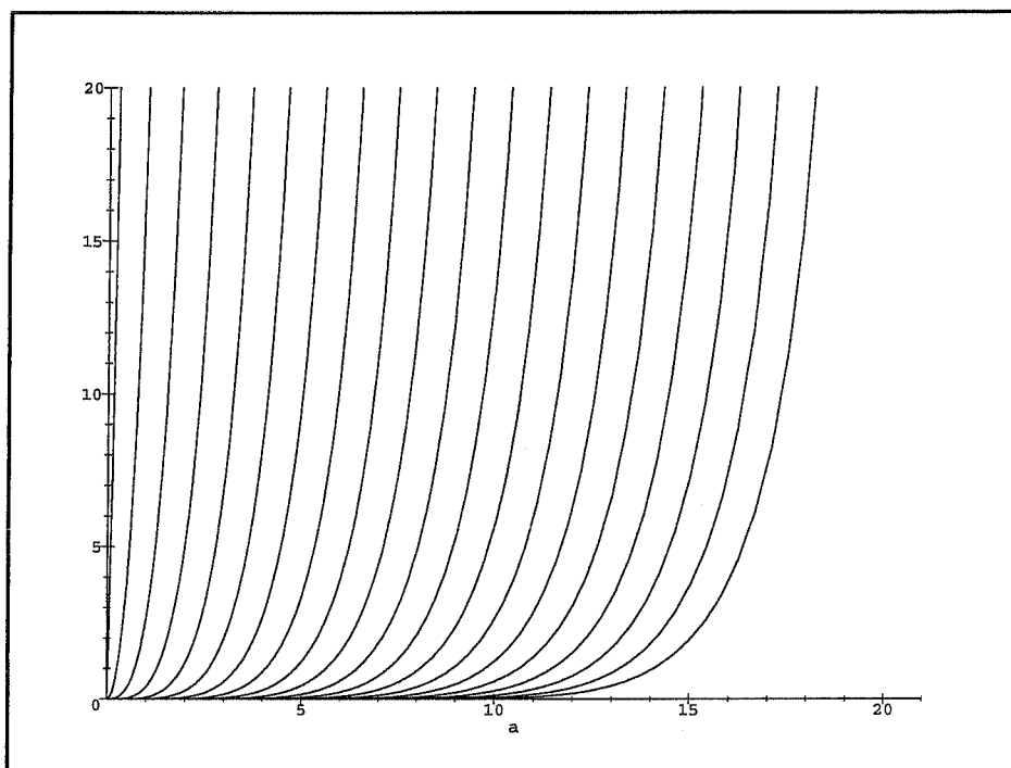
Values of \mathbb{E}W_Q as a function of the load a for (from left to right) s = 1 to 20 and \beta = 60 .
