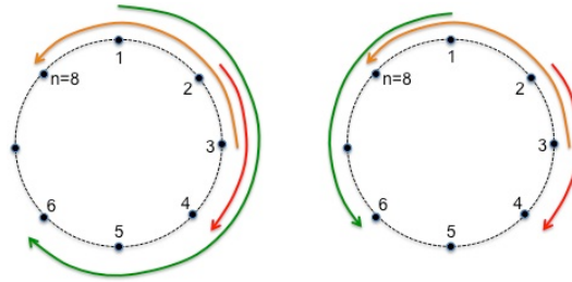
Figure 1: (For question 5) The instance in this example is given by n = 8 , C = \{c_1, c_2, c_3\} with c_1 = (1, 6) , c_2 = (2, 4) , and c_3 = (3, 8) . Left is a solution with value 3. Right is an optimal solution with value 2.
