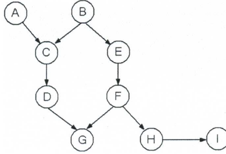
Figure 2: Graphical model.
